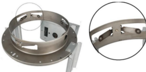
Fig. 33 Dual Point Retention Springs on Plaster Ring
