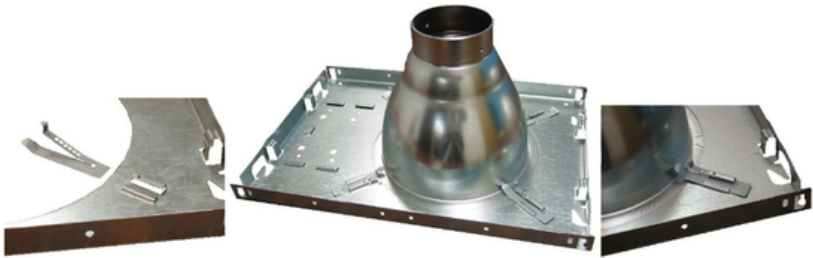
Fig. 32. 0043 Linear Clips on plaster frame 1431-X
