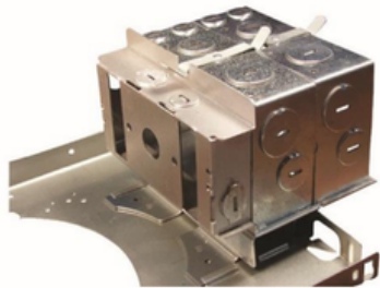
Fig. 44 1232 Junction Box with 3D Cover 1242-25B mounted to the inside (left) face, and Extender Box 1232E to the outside (right) face
