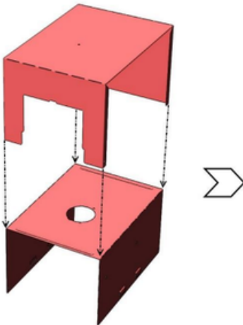
Fig. 52 Knockdown IC Box Exploded
