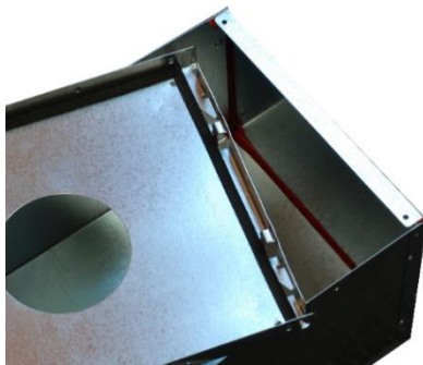
Fig. 47 1681-XX or 1685-XAT series Ultra-airtight IC Box (with integral gasketed junction box) with 1286-XAT series plaster frame mounted
