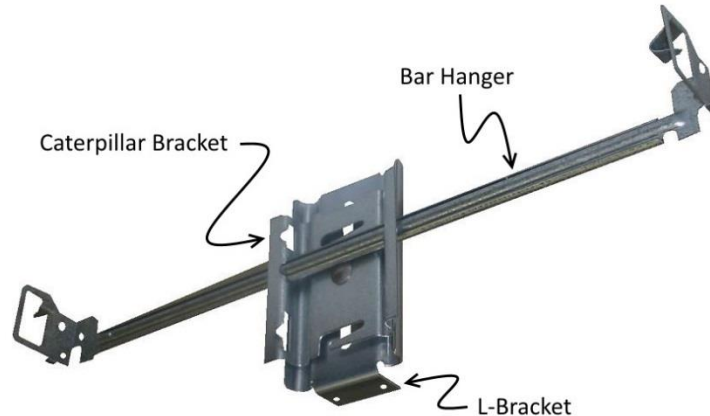
Fig. 65 Bar Hanger installed in #1054 Caterpillar Bracket/#1253-1 L-Bracket
