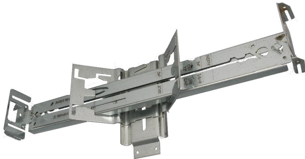
Fig. 64 #1487 L-Bars installed in #1254 Butterfly Bracket/#1253 (or 1253-4) Straight Bracket
