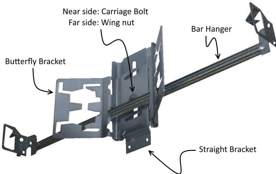
Fig. 63 #1287 Bar Hanger installed in #1254 Butterfly Bracket/#1253 (or 1253-4) Straight Bracket
