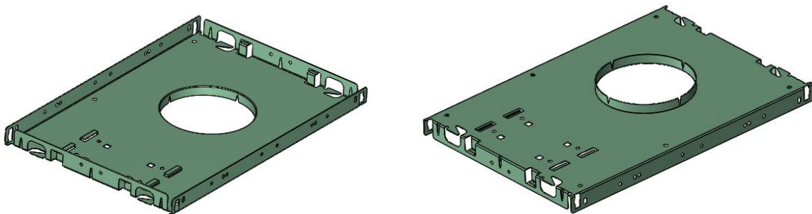
Fig. 19 Plaster frame with flanged hole & "gunsights"
