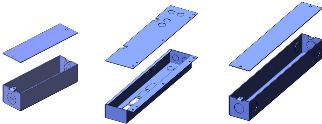
Fig. 68 Fixed length Driver Box & Cover
