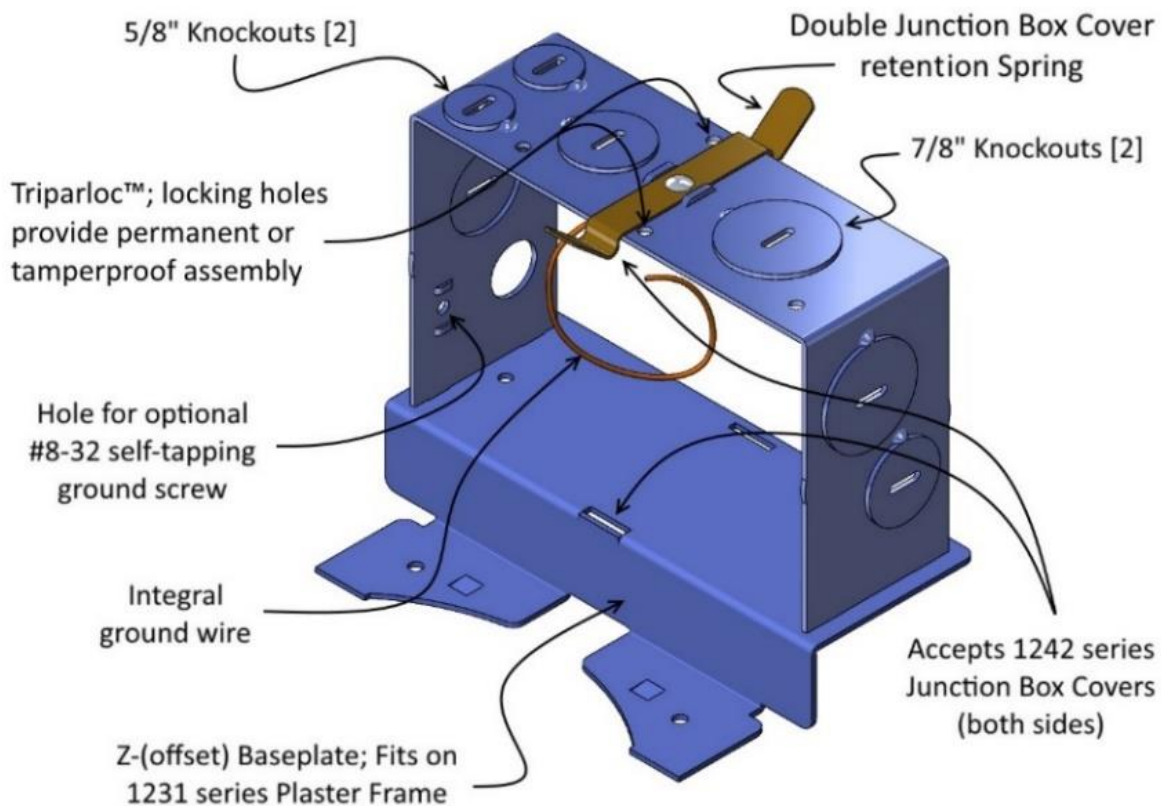
Fig. 39 Tripar's 1232-10 junction box
