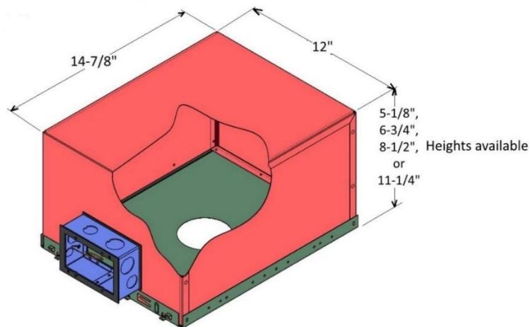
Fig. 49 1483-XAT series plaster frame mounted to 1682-XAT or 1684-XAT series Ultra-Airtight IC Box. Also available in black prepainted steel; see section 7.2.2.3
