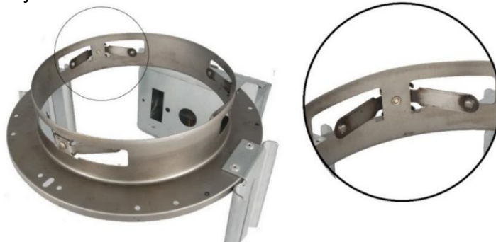
Fig. 33 Dual Point Retention Springs on Plaster Ring
