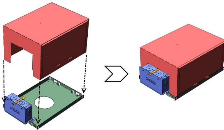
Fig. 45 Knockdown IC Box with J-box, Exploded (left) & Assembled (right)
