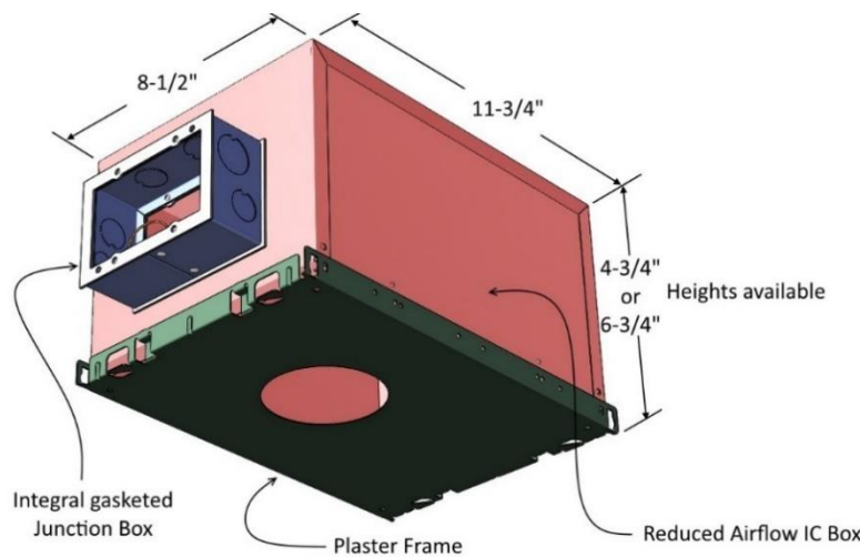
Fig. 48; 1681-XAT series Ultra-Airtight IC Box with integral gasketed junction box and 1286 series plaster frame
