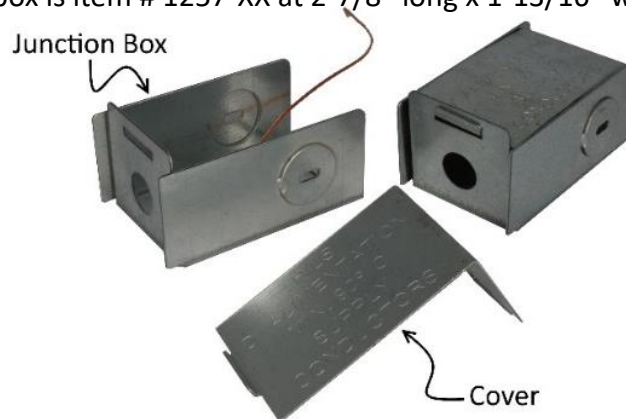
Fig. 42 1257-1 Junction Box & 1258 Cover
