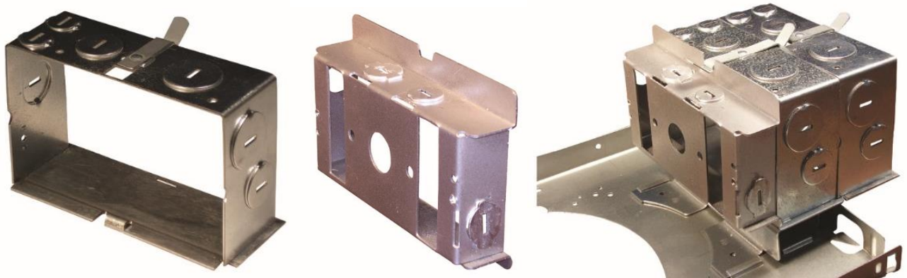
Fig. 40; Left Extender Box 1232E, Middle 3D Cover 1242-25B, Right 1232 Junction Box with 3D Cover 1242-25B mounted to the inside (left) face, and Extender Box 1232E to the outside (right) face
