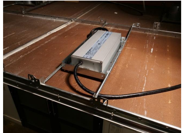
Fig. 26 #1405-6 with #1287 bar hangers installed in drop ceiling
