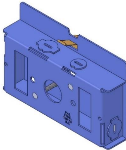
Fig. 56 Inner junction box 3D cover #1242-18B-AT (Suitable for only Standard size Airtight Junction Box 1281-92-1)
