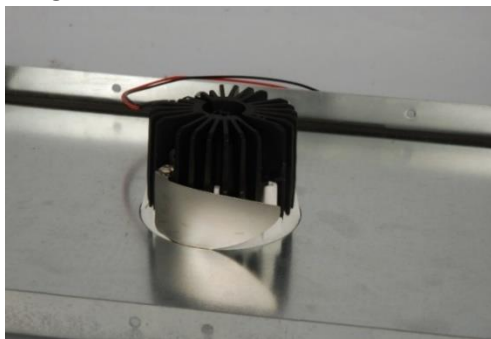
Fig. 34 Leaf Spring.
