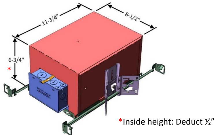
Fig. 46 Knockdown IC Box with Plaster Frame, J-box, Sliding Brackets, Butterfly Brackets, and bar hangers
