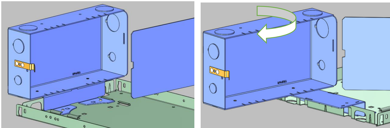
Fig. 41 1432 Junction Box (left) & 1432T junction box (right)
