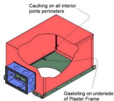
Fig. 47 1681-XX or 1685-XAT series Ultra-airtight IC Box (with integral gasketed junction box) with 1286-XAT series plaster frame mounted
