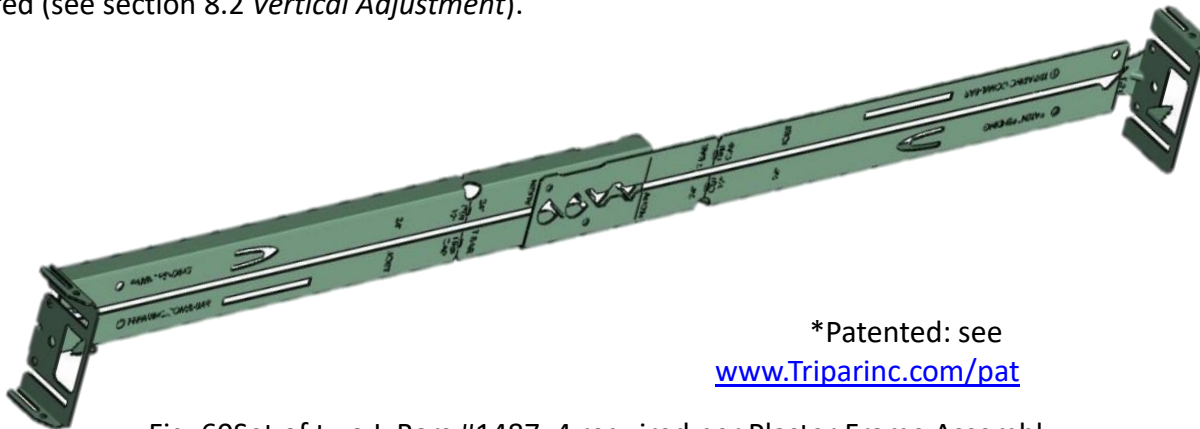
Fig. 60Set of two L-Bars #1487, 4 required per Plaster Frame Assembly
