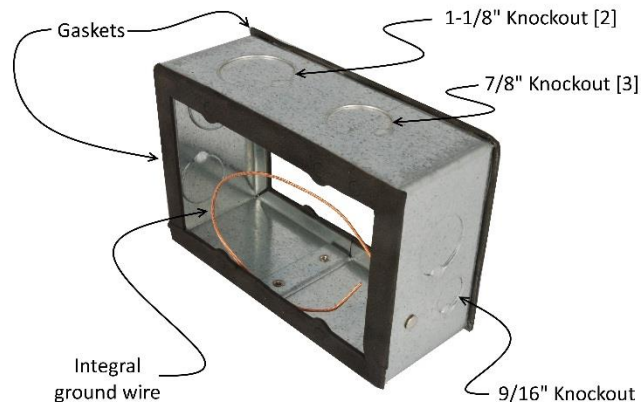
Fig. 53 Integral gasketed junction box used on Reduced Airflow & Ultra-Airtight IC Boxes
